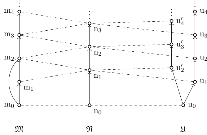
FIGURE 3. \mathfrak{N} and \mathfrak{M} are \downarrow -bisimilar but not quasi-injectively bisimilar; \mathfrak{N} and \mathfrak{U} are quasi-injectively bisimilar.
