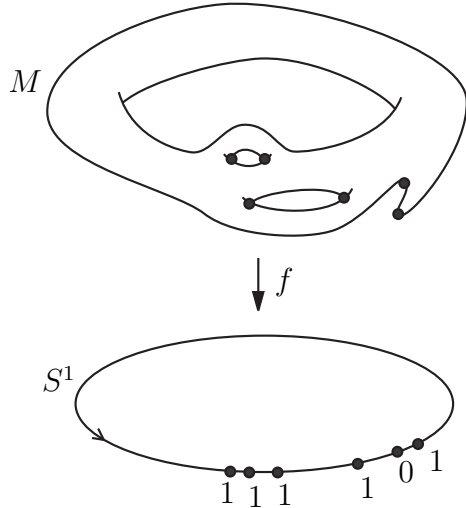
FIGURE 1. An example of a Morse map and the indices of its critical points
