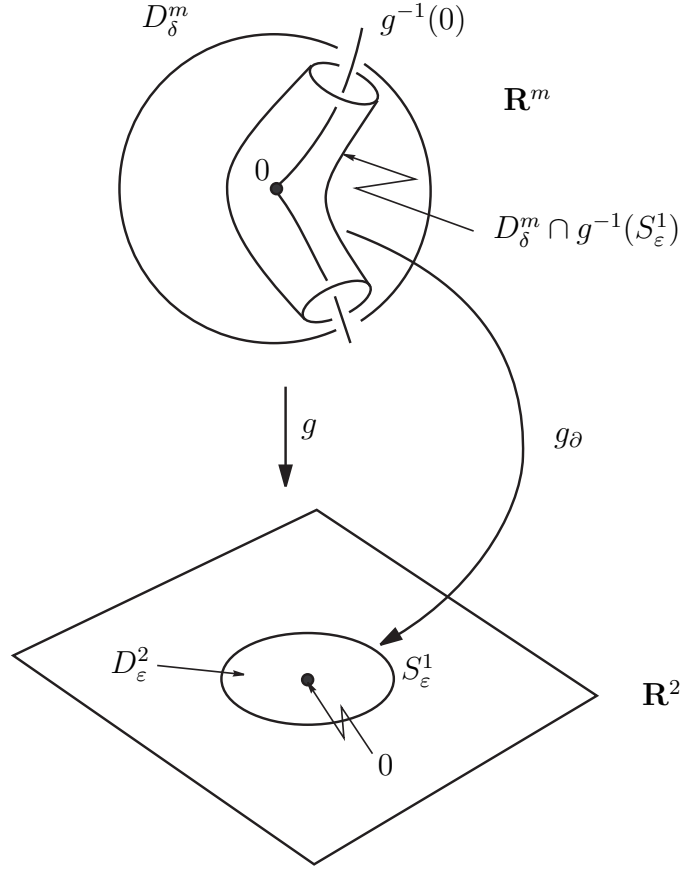
FIGURE 6. A generic map germ
