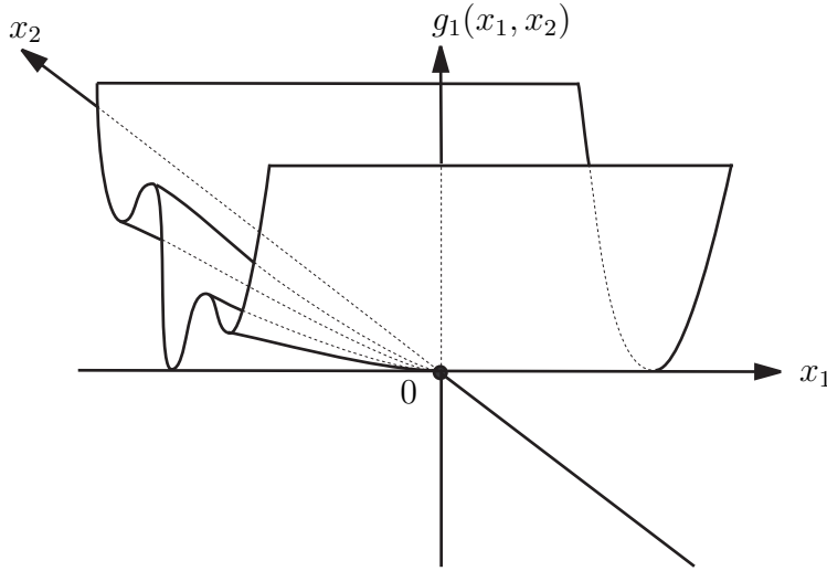
FIGURE 9. The graph of g_1(x_1, x_2)
