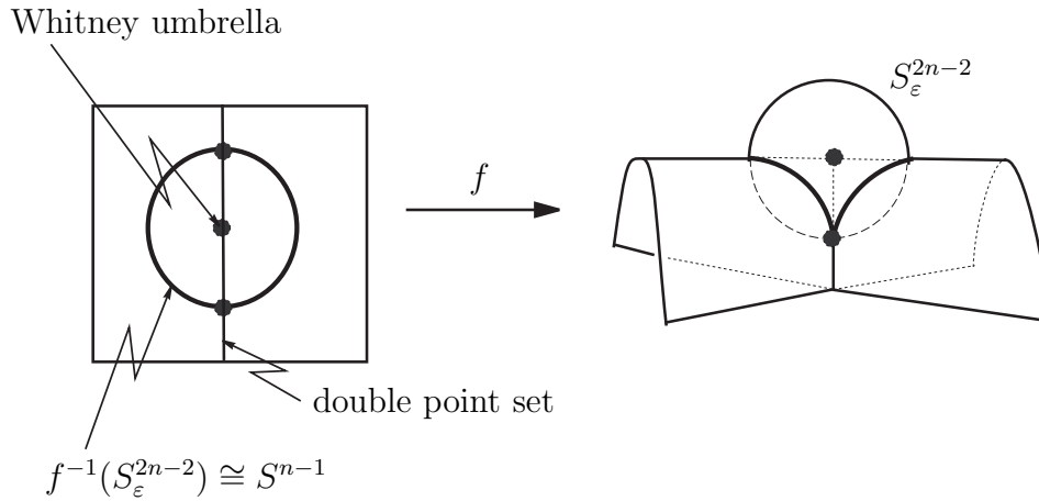
FIGURE 11. A Whitney umbrella and the associated immersion with a double point
