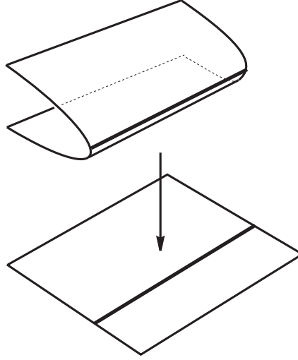
FIGURE 2. Map along a fold curve
