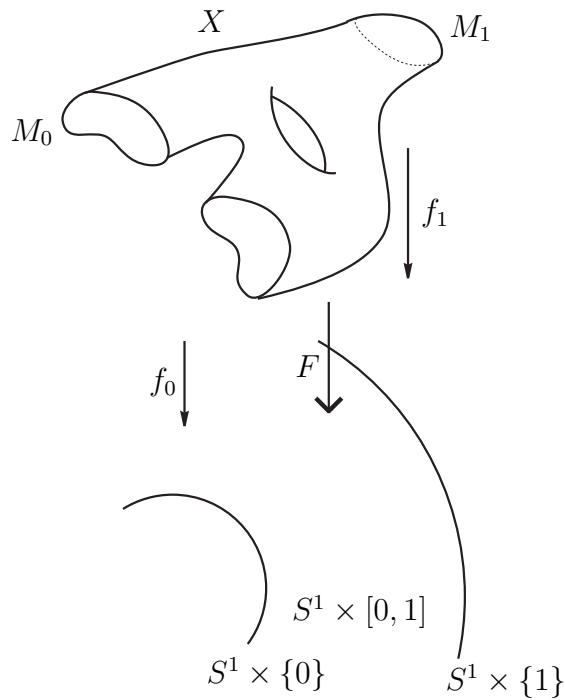
FIGURE 4. A fold cobordism
