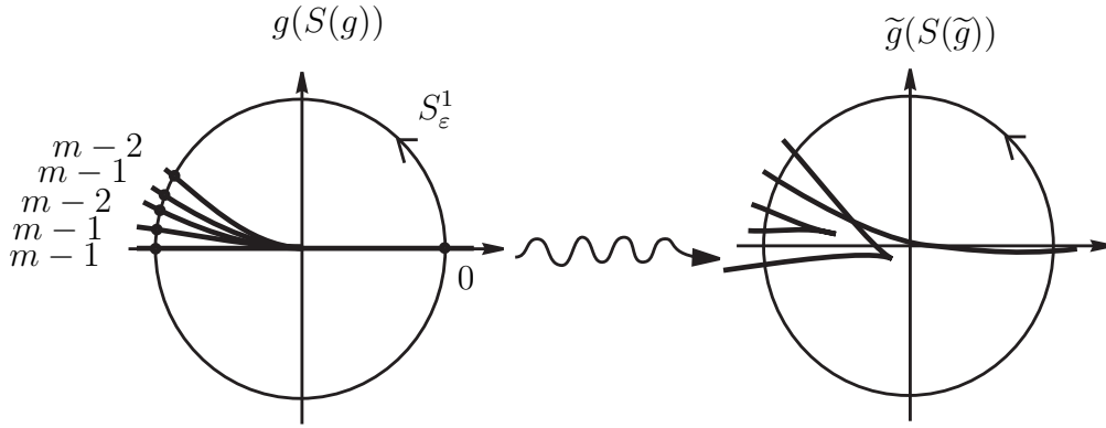
FIGURE 10. An example of a C^\infty stable perturbation of g
