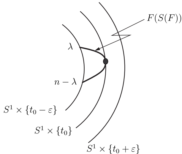
FIGURE 5. Fold cobordism invariance of C_\lambda - C_{n-\lambda}
