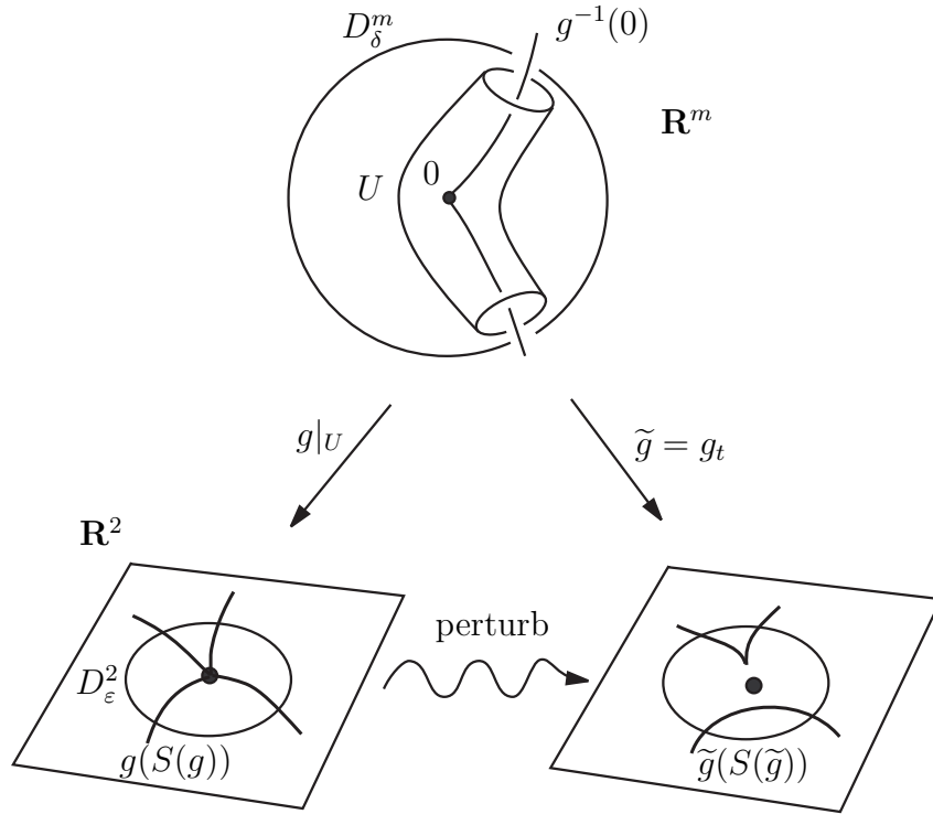
FIGURE 7. A C^\infty stable perturbation of a map germ
