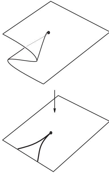
FIGURE 3. Map around a cusp
