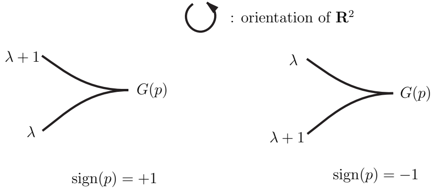
FIGURE 8. Indices of fold curves and the sign of a cusp point p of G
